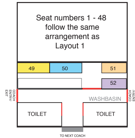
LAYOUT 2
